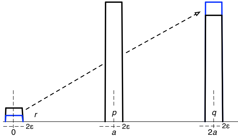
Figure A.1. : Figure for Axiom 5.
