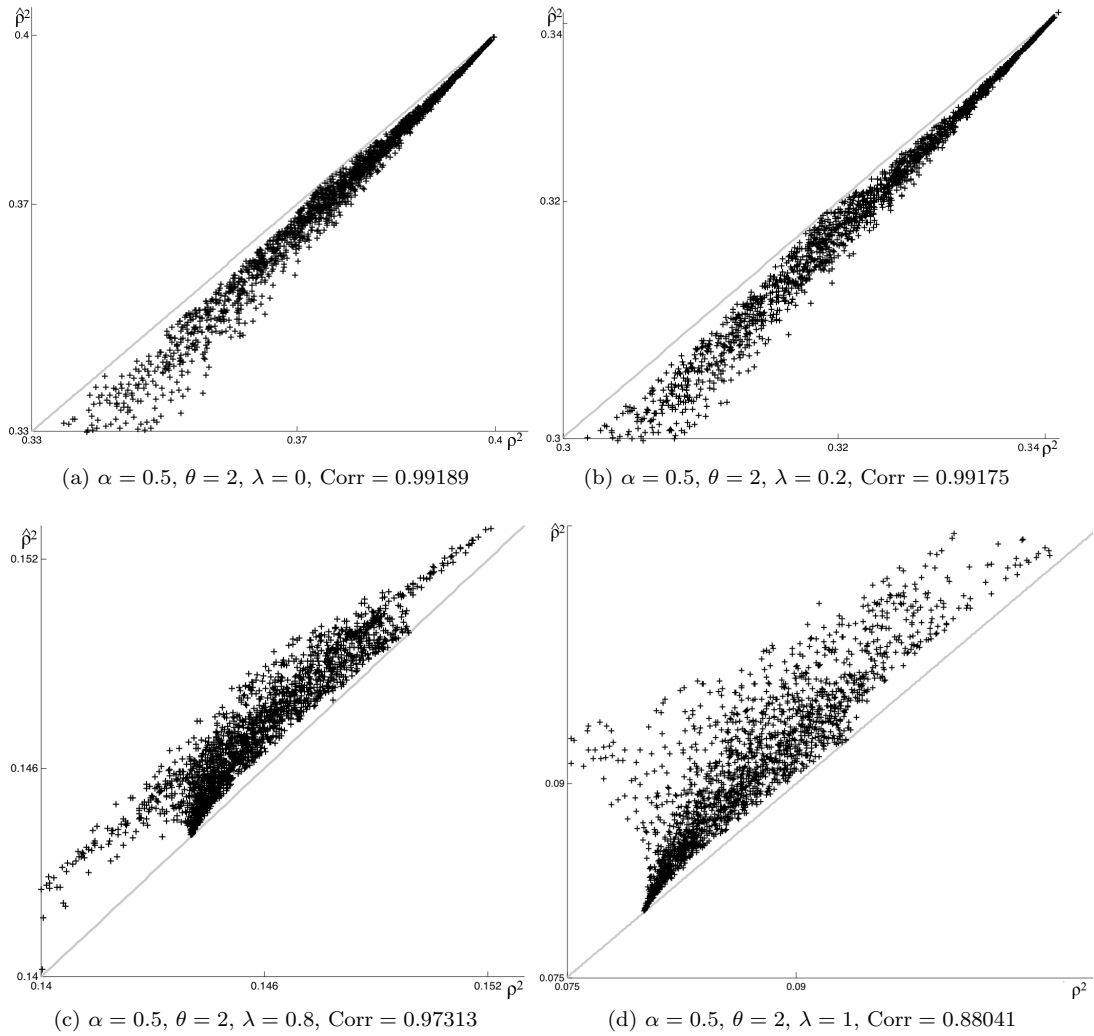
Figure 1. : THE PROXY MEASURE AND TRUE CONFLICT: BASELINE CASE
