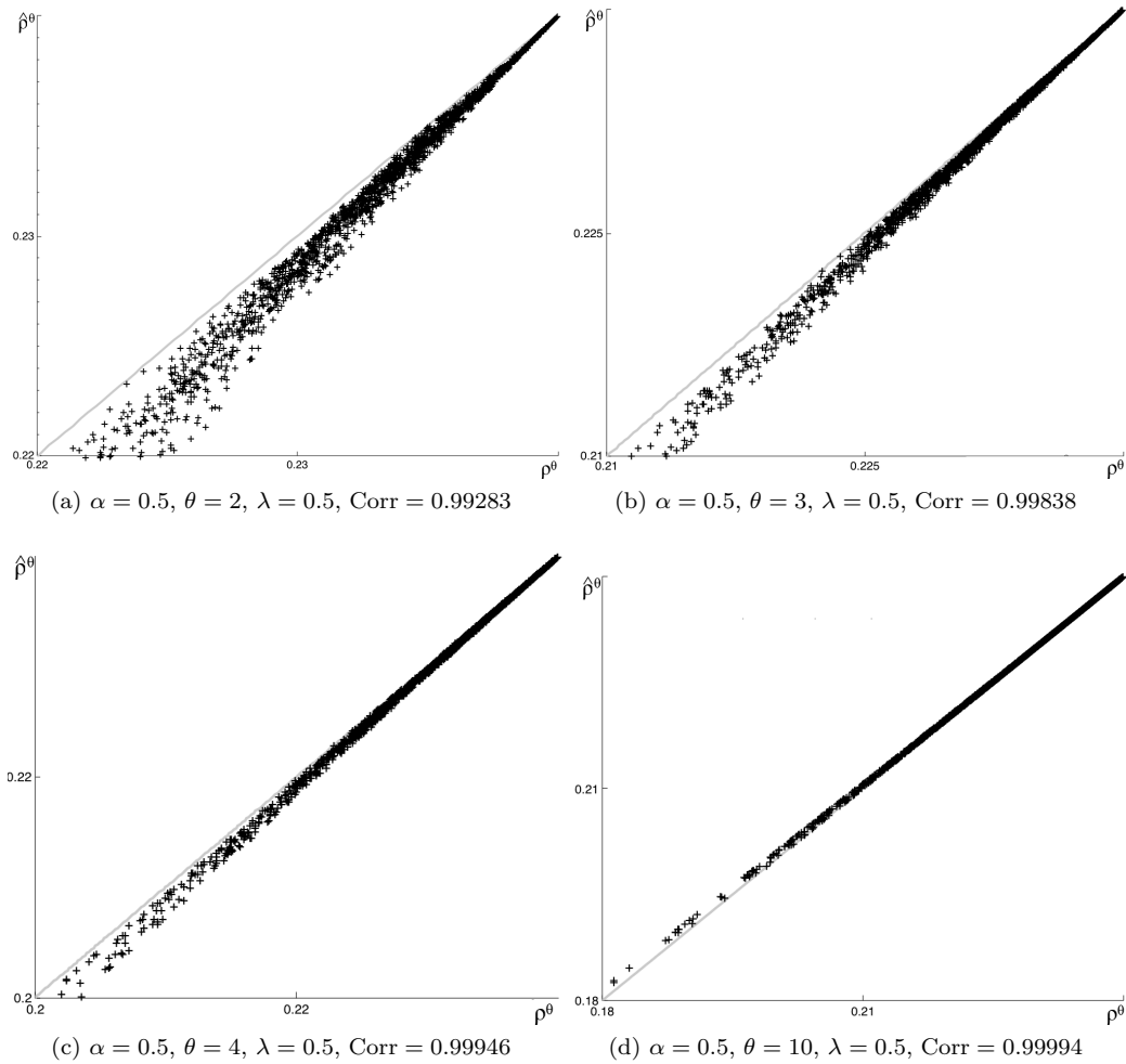
Figure 4. : THE PROXY MEASURE AND TRUE CONFLICT: NONQUADRATIC COSTS
