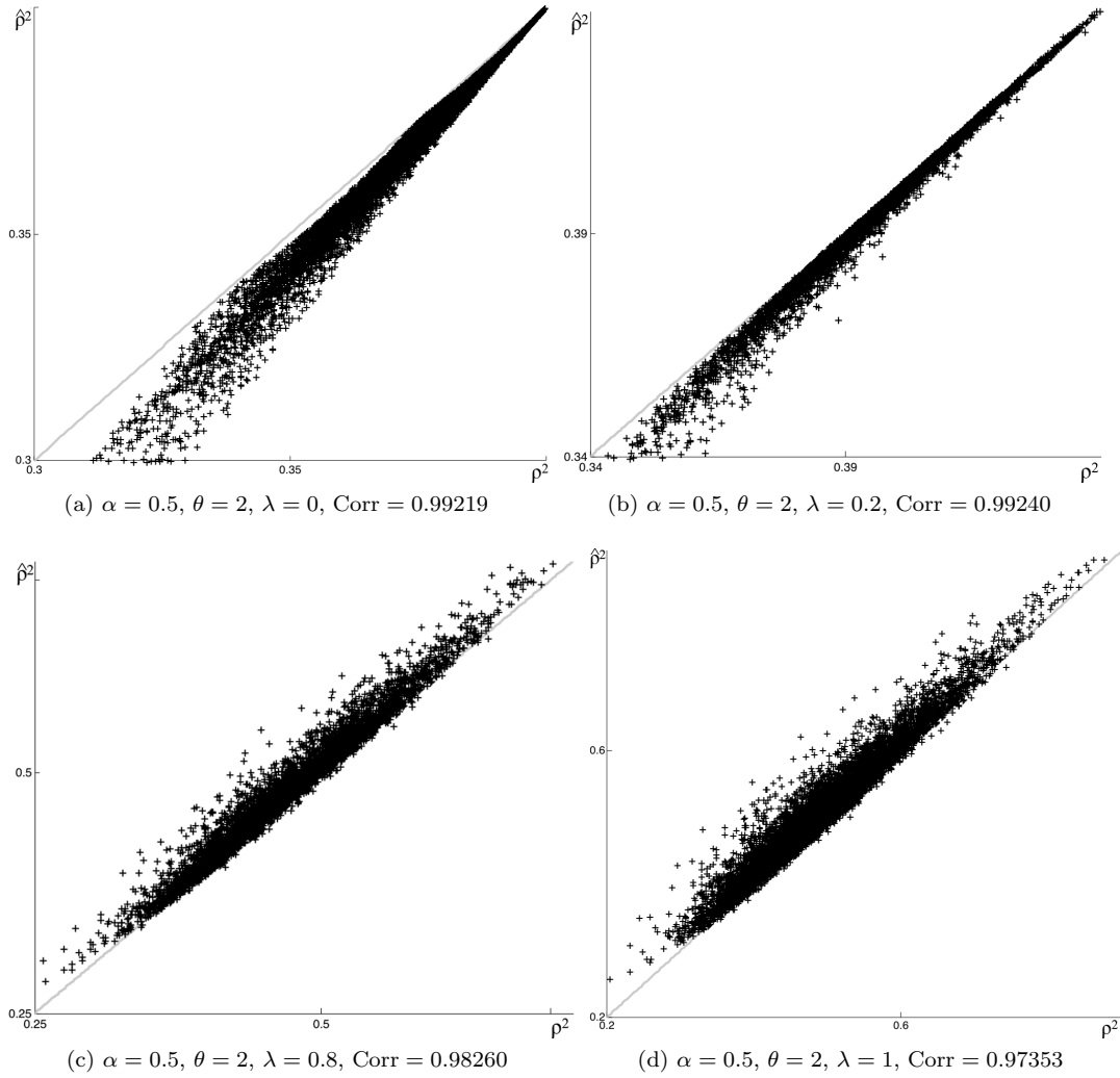
Figure 2. : THE PROXY MEASURE AND TRUE CONFLICT: VARYING UTILITY DISTANCES
